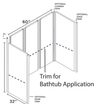
60" SHOWER/BATH 60" W X 32" D X 78" H 5 Panels | 7 Finishes
