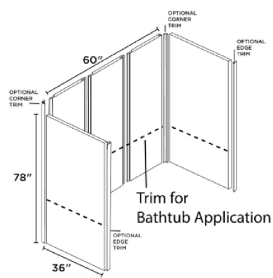
60" SHOWER/BATH 60" W X 36" D X 78" H 5 Panels | 4 Finishes
